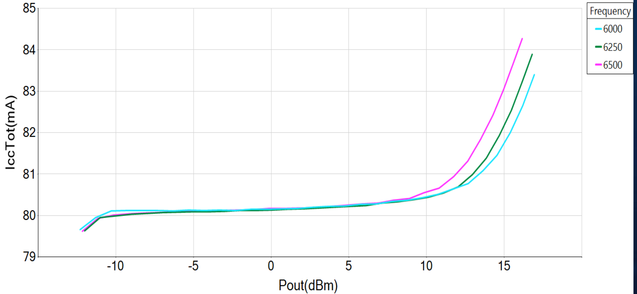
GRF2083 IccTot vs Pout at SerNum = 199
