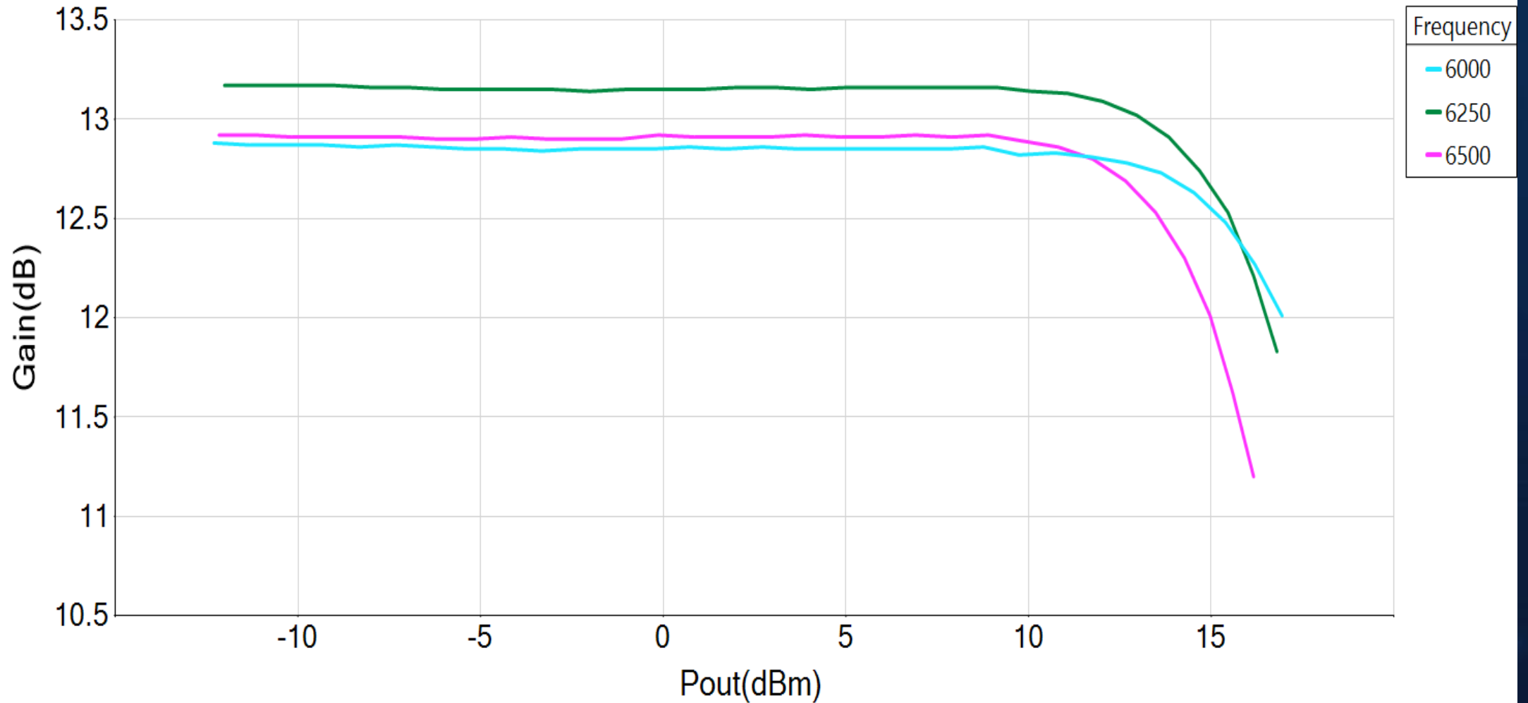
GRF2083 Gain vs Pout at SerNum = 199
